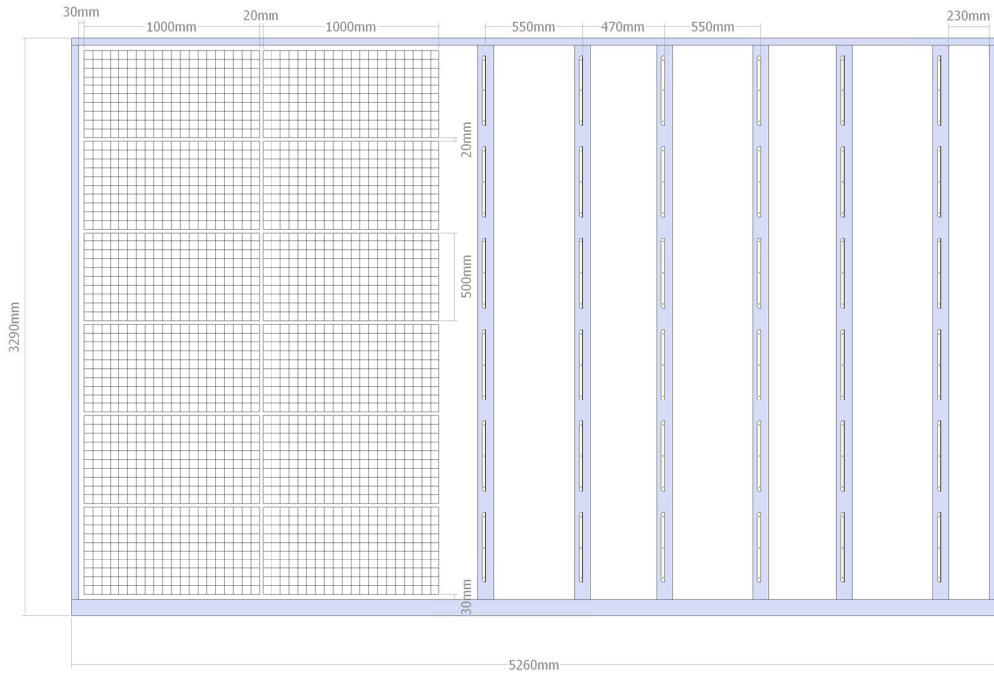
Front Elev.
