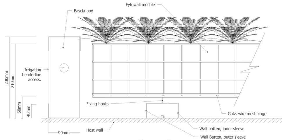
Plan - section
